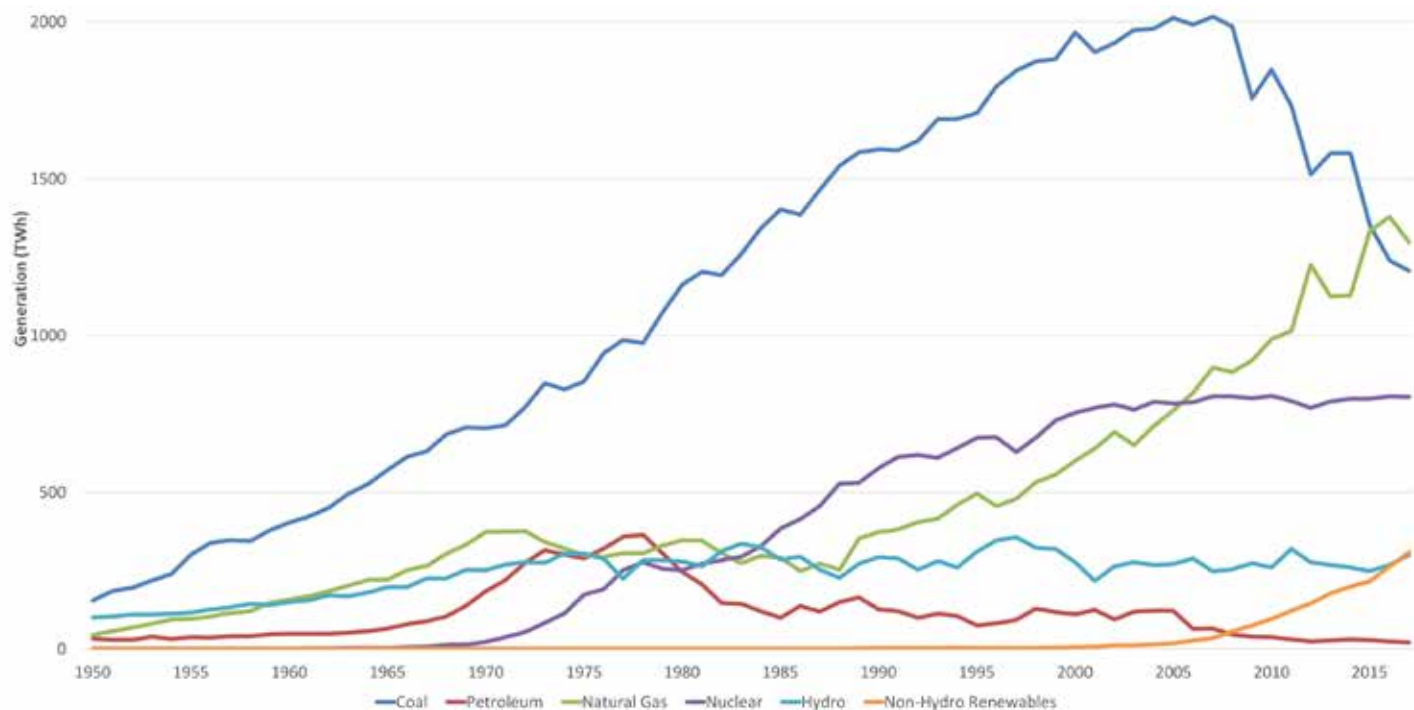
Figure 1. Historical Generation by Fuel Type, 1950–2016 (EIA 2016d).
